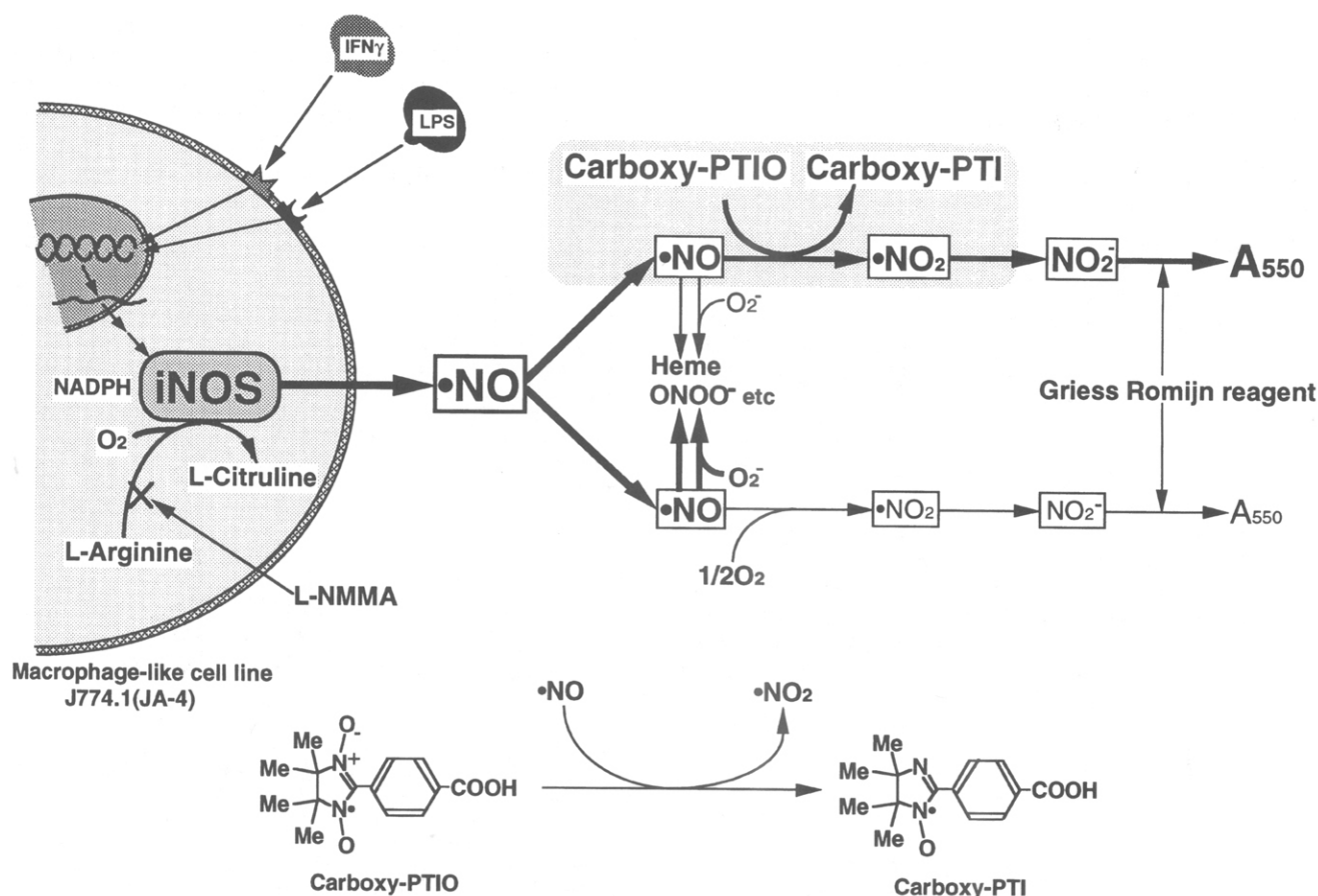
Fig. 1. A model of the enhancing effect of carboxy PTIO on the production of \text{NO}_2^- by an activated macrophage culture, and improvement of the detection of \text{NO}^* by the combined use of carboxy PTIO and Griess reagent.
